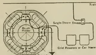
FIG. 2. CONNECTIONS FOR MAKING TEST ON INTERPOLE COILS.
